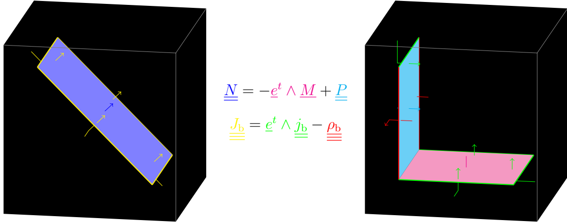
Figure A8.3.1: Space and time decomposition of \underline{\nabla} \wedge \underline{N} = \underline{J}_b and \underline{\nabla} \wedge \underline{J}_b = 0 to give \underline{\nabla}^{(3)} \wedge \underline{P} = -\underline{\rho}_b and -\underline{\nabla}^{(3)} \wedge (\underline{e}^t \wedge \underline{M}) + \underline{e}^t \wedge \underline{\dot{P}} = \underline{e}^t \wedge \underline{j}_b and -\underline{\nabla}^{(3)} \wedge (\underline{e}^t \wedge \underline{j}_b) + \underline{e}^t \wedge \underline{\dot{\rho}}_b = 0 . One external space dimension has been suppressed.
