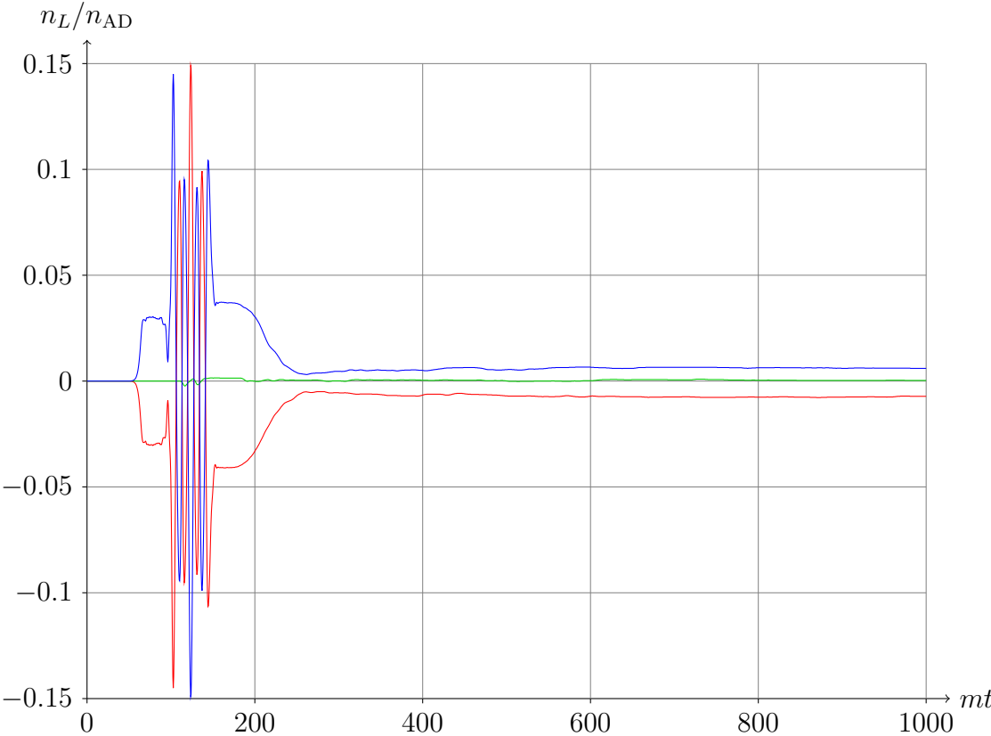
Figure 1.3: Lepton number generated at the end of thermal inflation.
