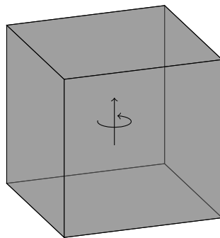
Figure 1.2: An oriented 3-volume.
